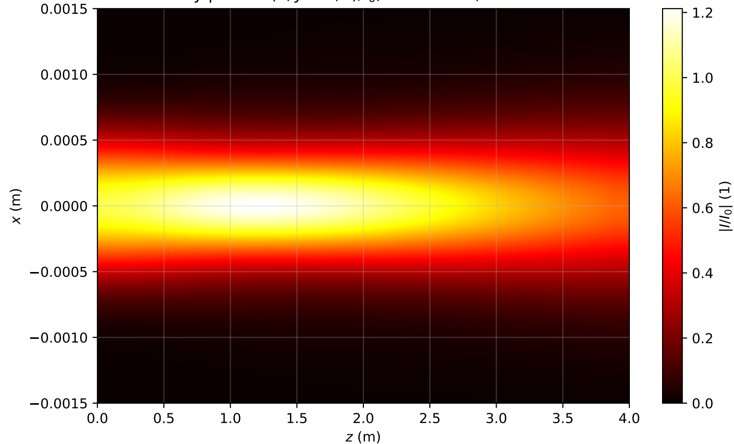
Intensity profile I(x, y = 0, z)/I_0 , P_{in}=0.7P_{cr} , artificial time
